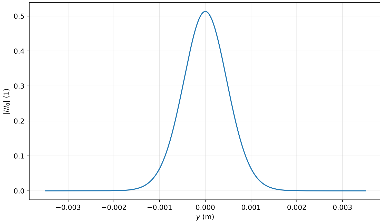
Intensity profile I(x=0, y, z=2.309)/I_0 , P_{in}=0.2P_{cr} , artificial time
